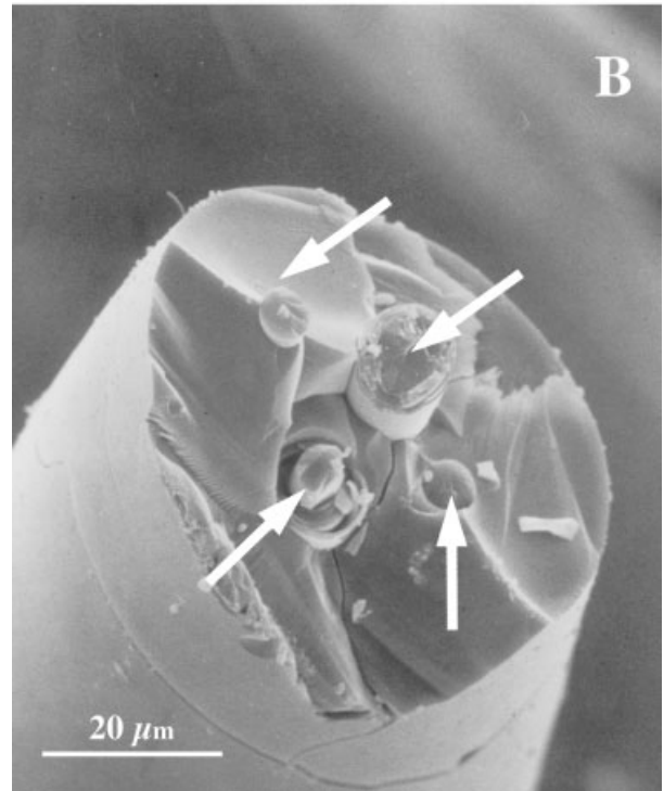
Fig. 12. SEM photograph of hexactinellid spicules embedded in silica. A: Partially embedded spicule (arrow). B: transversal section showing spicules (arrows) surrounded by large amounts of additional silica.
